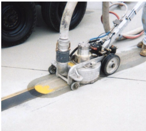
Lines Stripe Removal using ultra-high waterblasting – approved for lead paint removal
